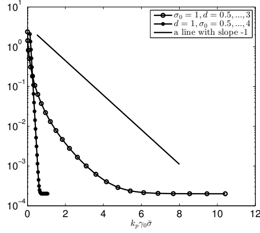
FIGURE 7.2. The \log \|\mathbf{u} - \mathbf{u}_h\|_{H^1(\Omega_l)} - k_p \gamma_0 \bar{\sigma} plot of the finite element solution \mathbf{u}_h when h = 1/128 and the degrees of freedom \text{DOF} = 8266752 .
