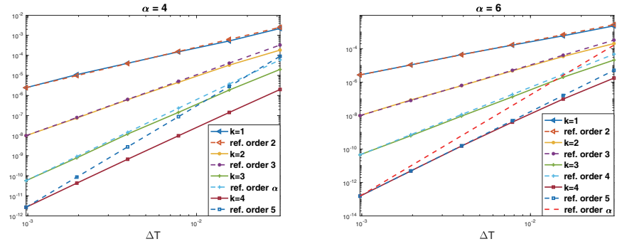
FIG. 3. Orders of convergence of the error in the \|\cdot\|_2 -norm sense with respect to \Delta T , for \bar{\alpha} = 4 (left) and \bar{\alpha} = 6 (right), for different values of k \in \{1, 2, 3, 4\} , in the linear implicit Euler scheme case.
