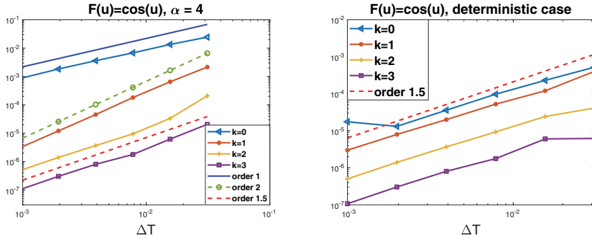
FIG. 4. Orders of convergence of the error in the \|\cdot\|_2 -norm sense with respect to \Delta T , for the additive noise case with \bar{\alpha} = 4 (left) and the deterministic case (right), for nonlinear F(u) = \cos(u) and different values of k \in \{0, 1, 2, 3\} , in the linear implicit Euler scheme case.
