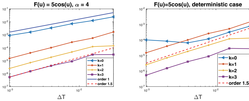
FIG. 5. Orders of convergence of the error in the \|\cdot\|_2 -norm sense with respect to \Delta T , for the additive noise case with \bar{\alpha} = 4 (left) and the deterministic case (right), for nonlinear term F(u) = 5 \cos(u) and different values of k \in \{0, 1, 2, 3\} , in the linear implicit Euler scheme case.
