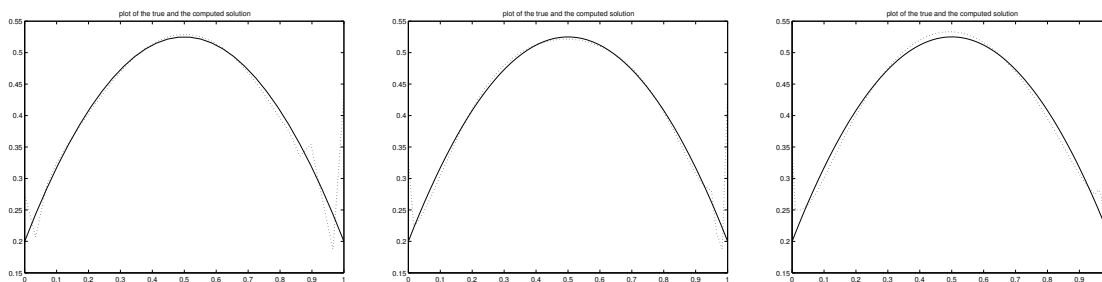
Figure 1. Solutions of the inverse gravimetry problem. Solid line: the true solution, x_{true} ; Dashed line: the approximate solution, x_{appr}
