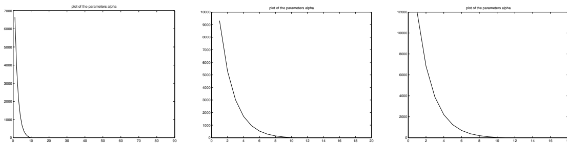
Figure 3. Last values of parameters \alpha in each iteration
