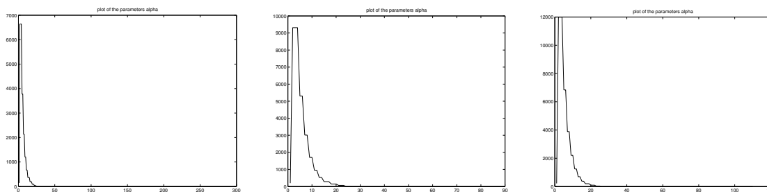
Figure 2. Parameters \alpha generated by Algorithm 4.1
