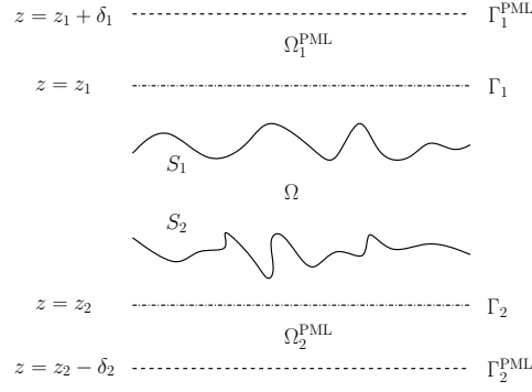
FIG. 5.1. Geometry of the PML problem.
