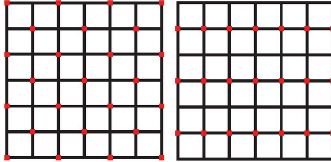
Figure 6.10: C/F splitting for the 2D elliptic problem with \epsilon = 1 (left) and \epsilon \ll 1 (right), where the red points are C-variables and the black points are F-variables.
