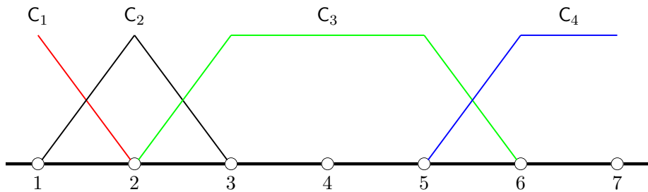
Figure 6.11: Aggregates and prolongation corresponding to (6.17).
