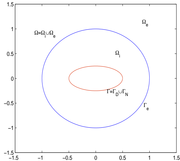
FIGURE 1. The artificial boundary
