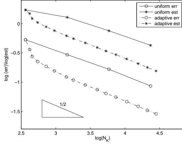
FIGURE 4. Convergence behavior for Example 1.
