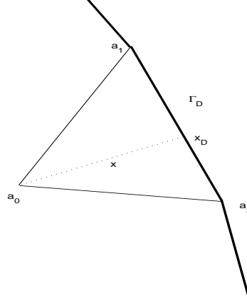
FIGURE 3. The element near \Gamma_D
