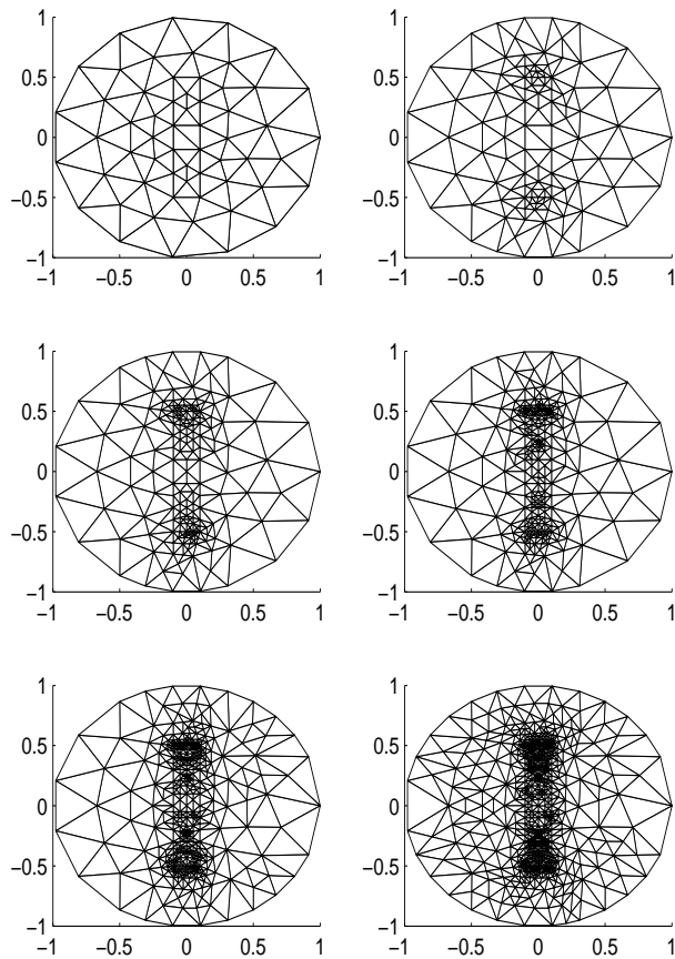
FIGURE 6. the mesh for Example 2.
