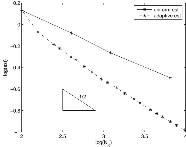
FIGURE 5. The convergence behavior for Example 2.
