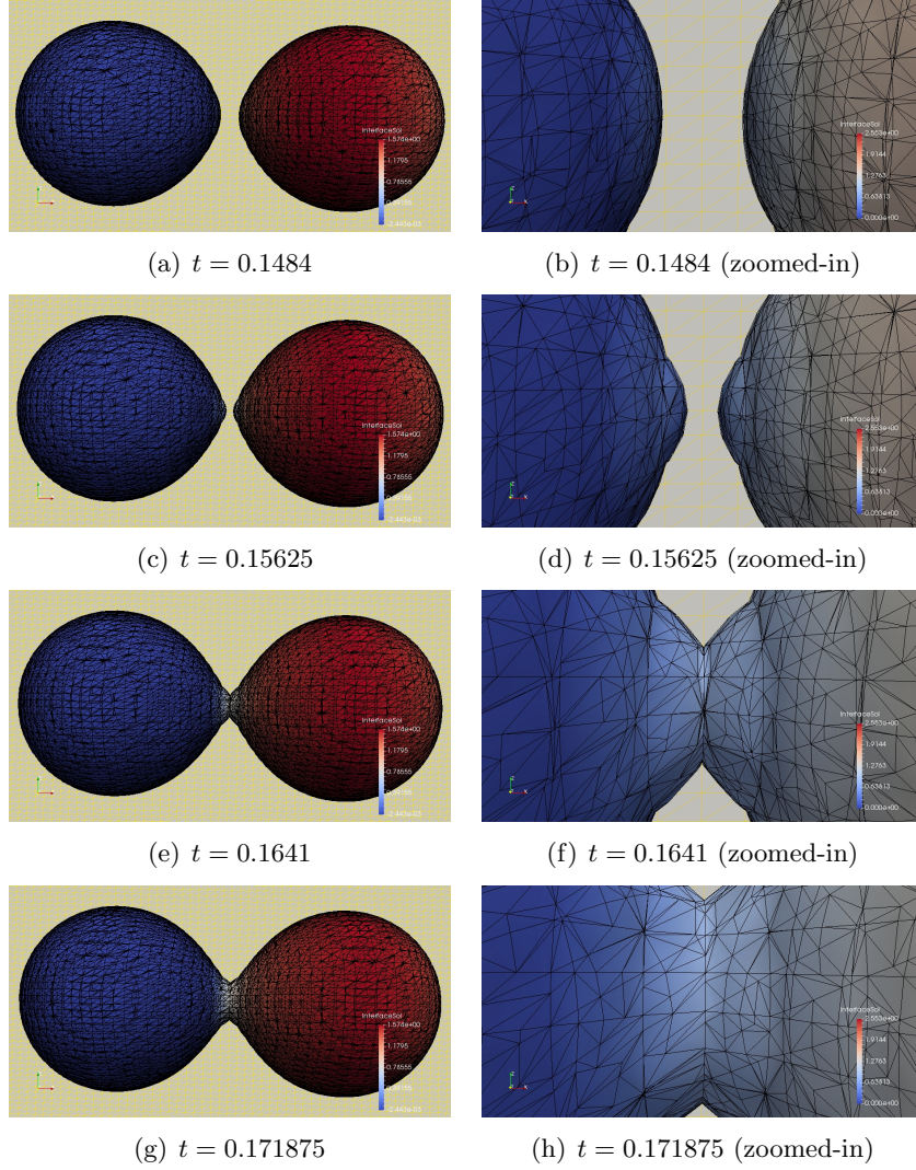
Figure 6: The computed solution and surface meshes close to the time of collision Example 5.
