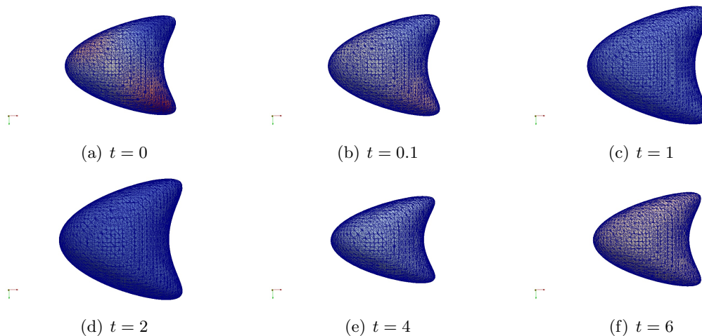
Figure 3: Snapshots of the surface, surface mesh and the computed solution from Experiment 4.
