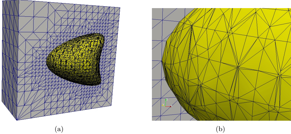
Figure 1: Left: Cutaway of the background and induced surface meshes for \Gamma_h(0) from Experiment 4 in Section 4. Right: The zoom-in of the surface mesh.
