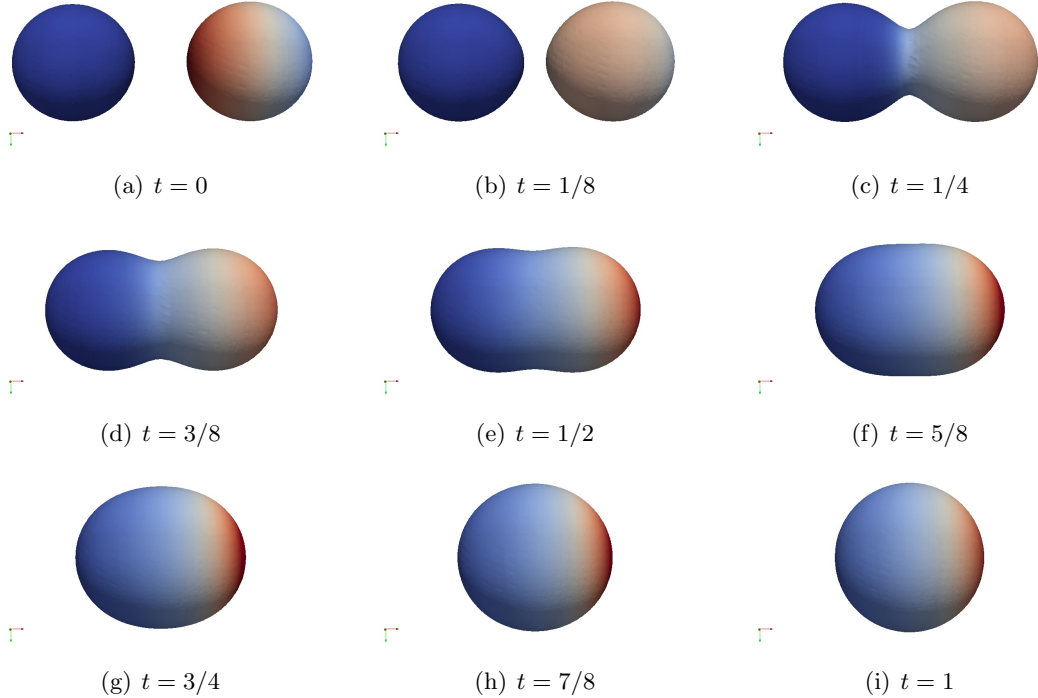
Figure 5: Snapshots of discrete solution in Experiment 5 with h = 1/16 , \Delta t = 1/128 .
