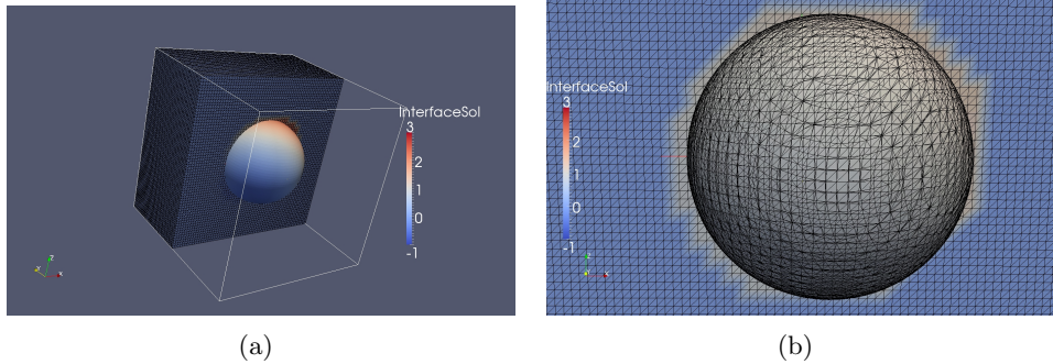
Figure 2: The cutaway of the background mesh and a part of the surface mesh for t_n = 1 . Colors illustrate the solution and its extension.
