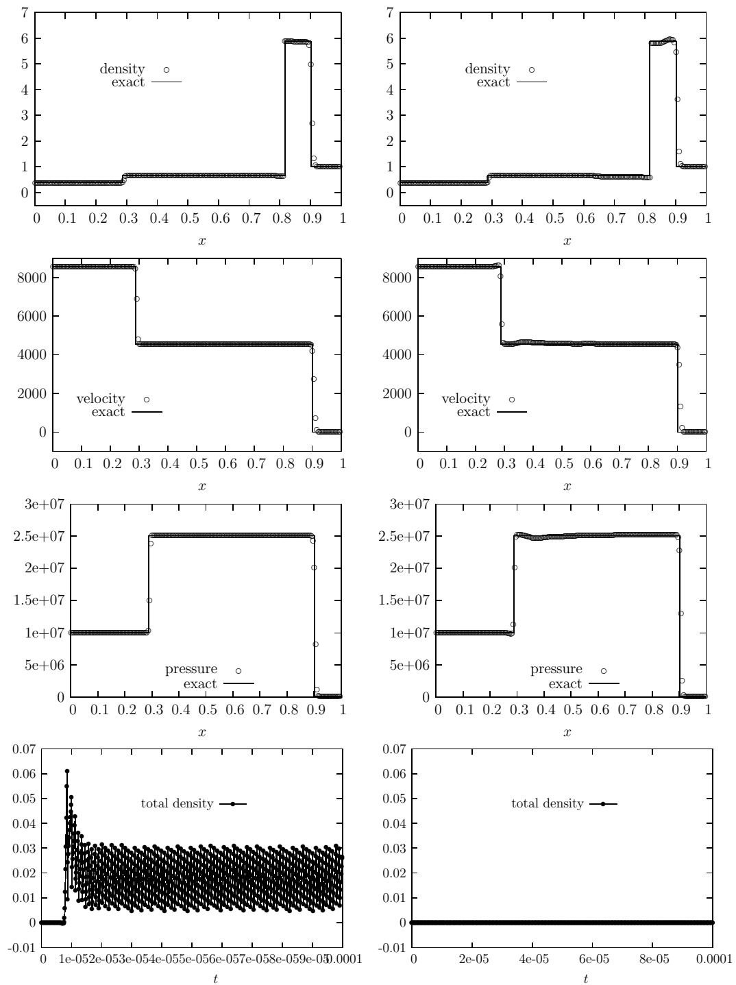
Figure 9: Example 4.6. Left: Result of GFM; Right: GFM with partially conservative modification. CFL=0.4.
