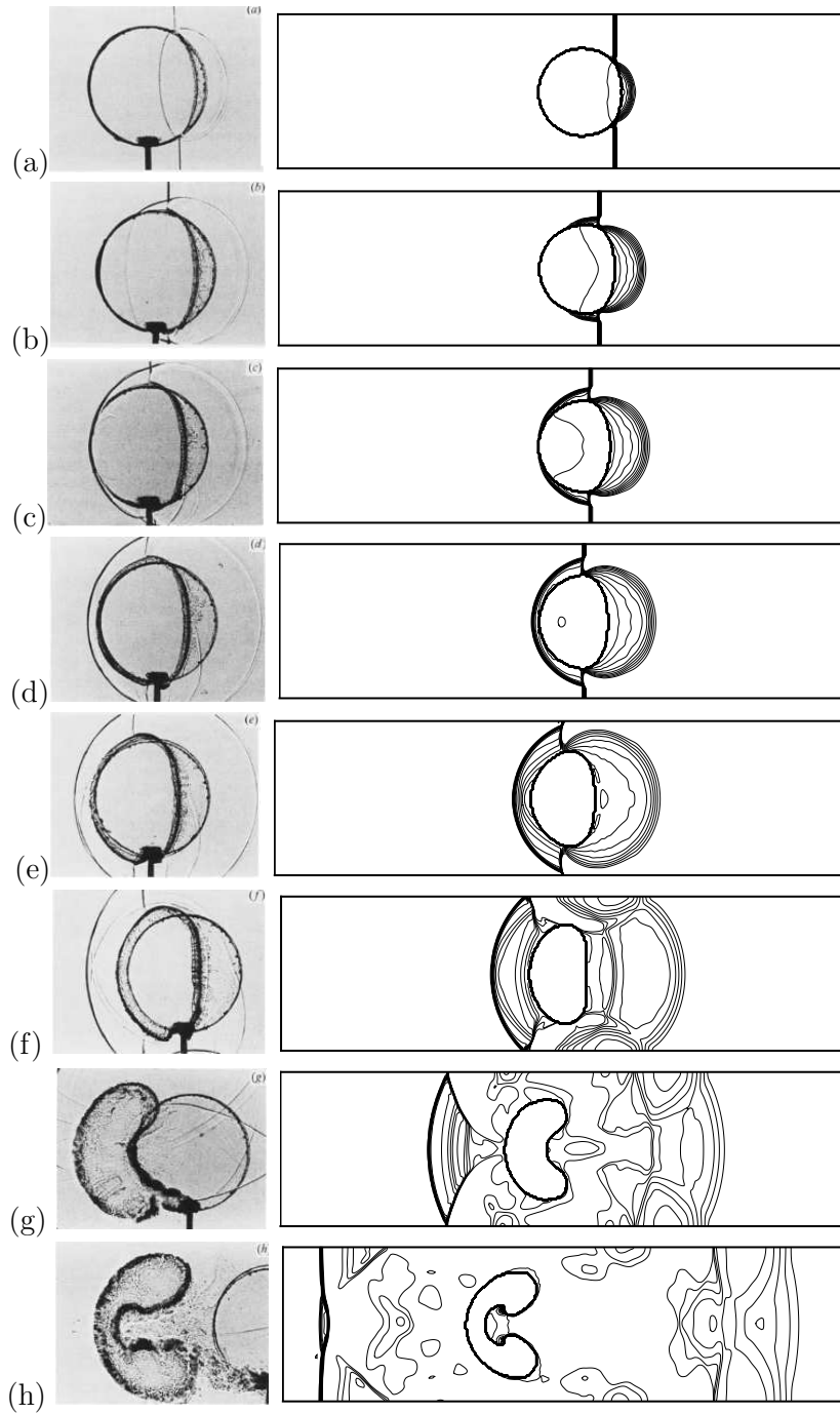
Figure 12: Example 4.8. Left: experimental result (Haas and Sturtevant [10]); Right: contour of density obtained by our partially conservative modified GFM. (a) t = 32\mu s , (b) t = 52\mu s , (c) t = 62\mu s , (d) t = 72\mu s , (e) t = 82\mu s , (f) t = 102\mu s , (g) t = 245\mu s , (h) t = 427\mu s .
