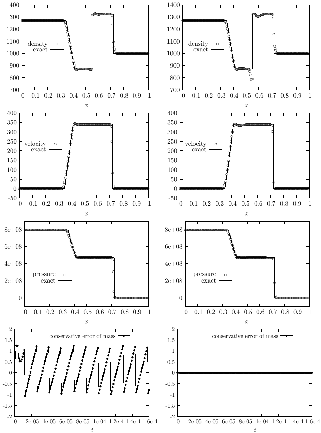
Figure 7: Example 4.4. Left: Result of GFM; Right: GFM with partially conservative modification. CFL=0.4.
