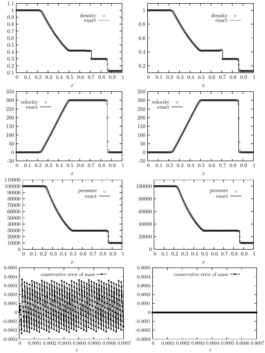
Figure 4: Example 4.1. Left: Result of GFM; Right: Result of GFM with partial conservative modification. CFL=0.4.
