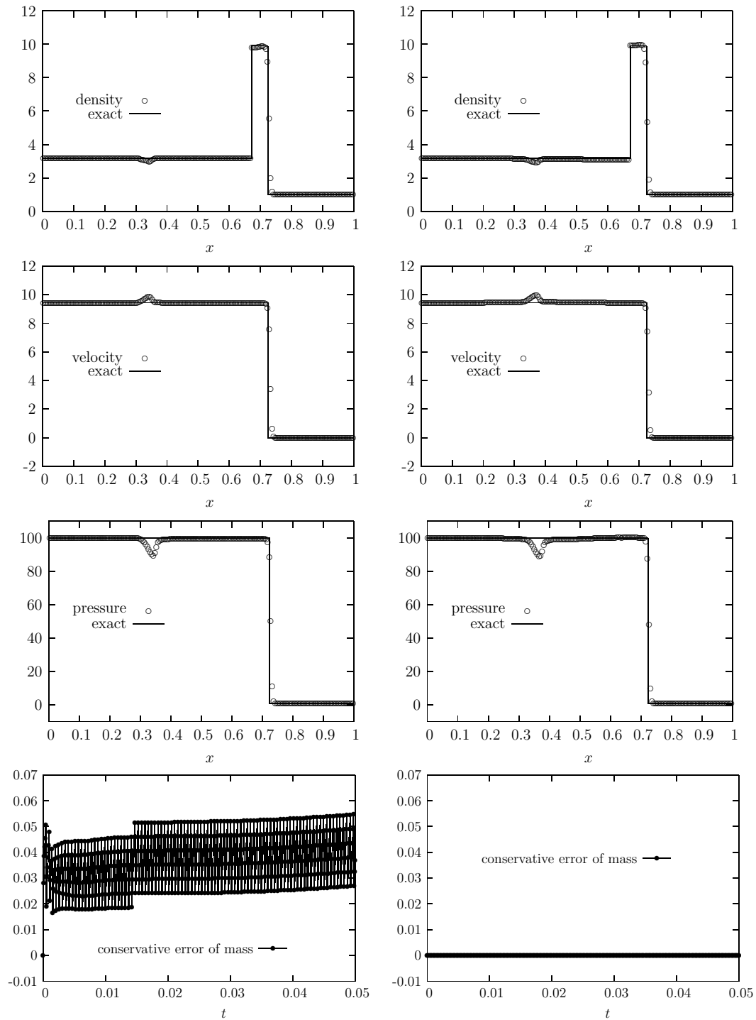
Figure 10: Example 4.7. Left: Result of GFM; Right: GFM with partially conservative modification. CFL=0.4.
