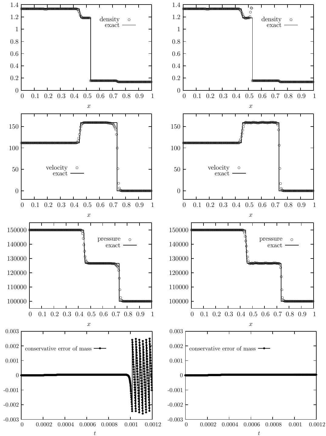
Figure 5: Example 4.2. Left: Result of GFM; Right: GFM with fully conservative modification. CFL=0.4.
