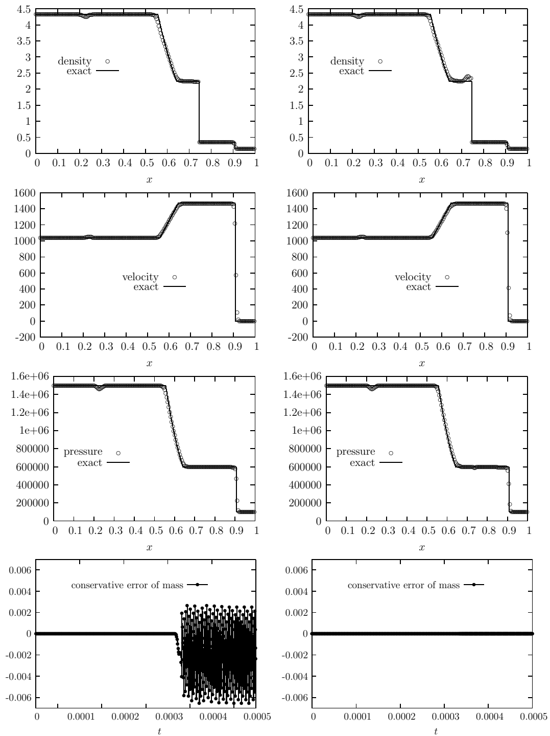
Figure 6: Example 4.3. Left: Result of GFM; Right: GFM with fully conservative modification. CFL=0.4.
