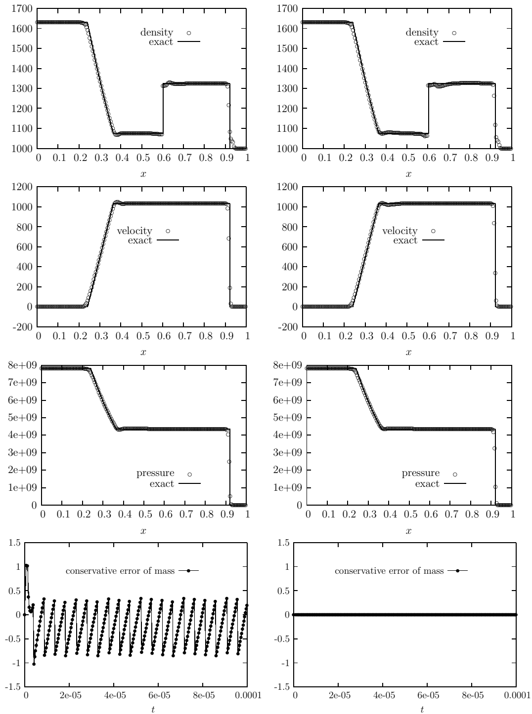
Figure 8: Example 4.5. Left: Result of GFM; Right: GFM with partially conservative modification. CFL=0.4.
