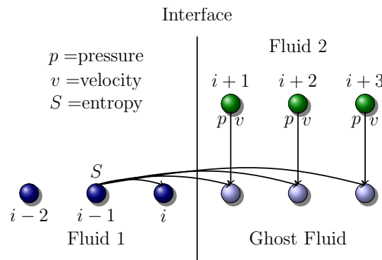
Figure 1: Ghost fluid method.
