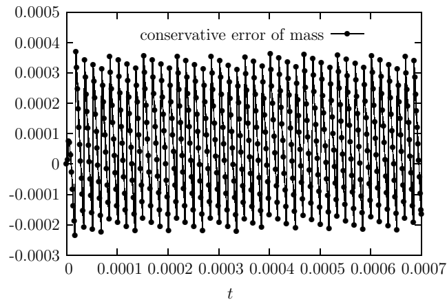
Figure 2: Mass conservation error of the two-phase Sod's shock tube problem using GFM.
