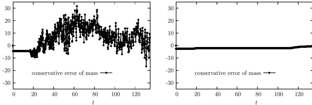
Figure 11: Example 4.8. Conservation errors of mass. Left: the GFM; Right: the partially conservative modified GFM.
