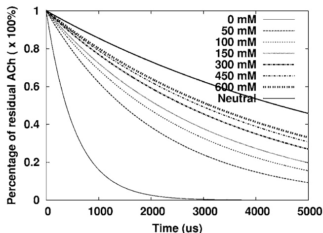
FIG. 12. Consumption of bulk ACh by the AChE monomer at different ionic strengths.
